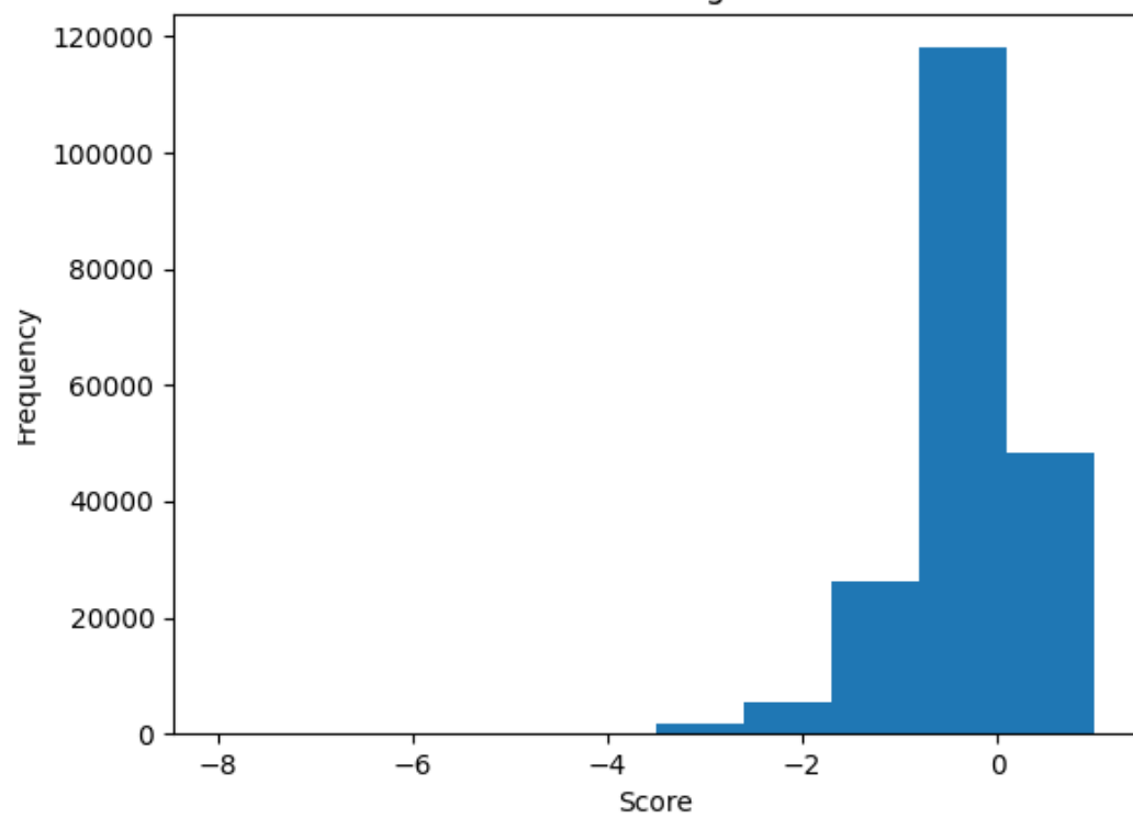
Score Histogram
